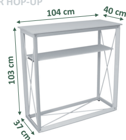
COMPTOIR HOP-UP
